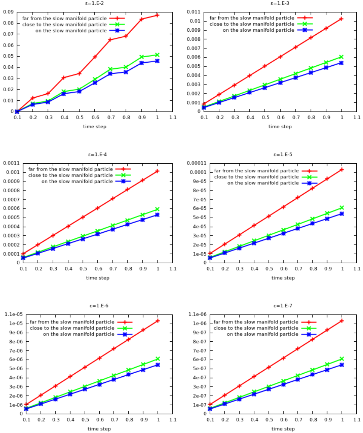
Figure 6: Global Euclidean errors of the ETD-PIC method at time 2\pi/a_\varepsilon \sim 1/\varepsilon for several values of \varepsilon , obtained with three initial conditions differently positioned with regard to the slow manifold \mathcal{D}_2
