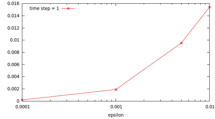
Figure 8: The difference between the density of the Vlasov-Poisson reference solution and the solution to the Guiding Center equation as a function of \varepsilon at final time t = 4 .
