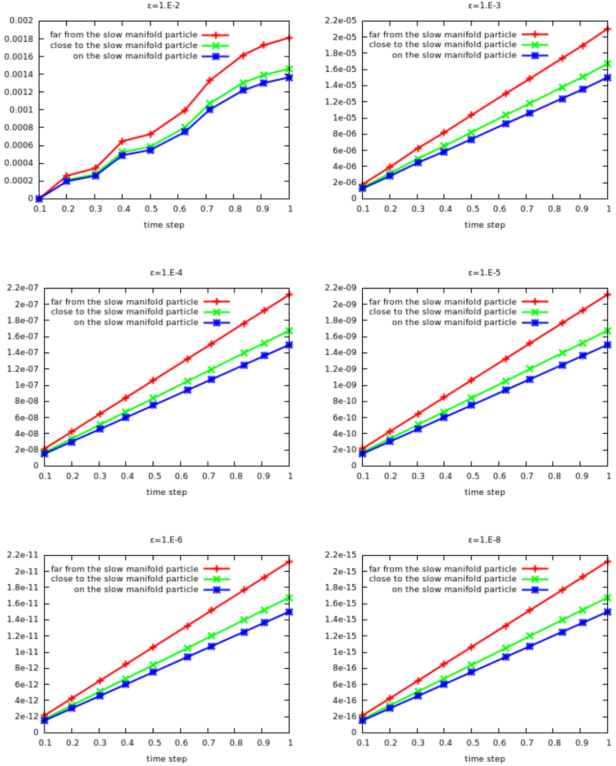
Figure 4: Global Euclidean errors of the ETD-PIC method at final time 10 for several values of \varepsilon , obtained with three initial conditions differently positioned with regard to the slow manifold \mathcal{D}_2 .
