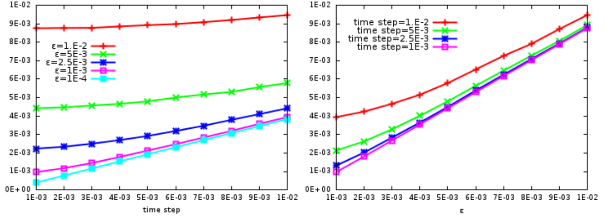
Figure 10: The difference between the solution computed with the ETD-PIC method and the solution to the Guiding Center equation as a function of the time step ( left panel) and of \epsilon ( right panel) at final time t = 5
