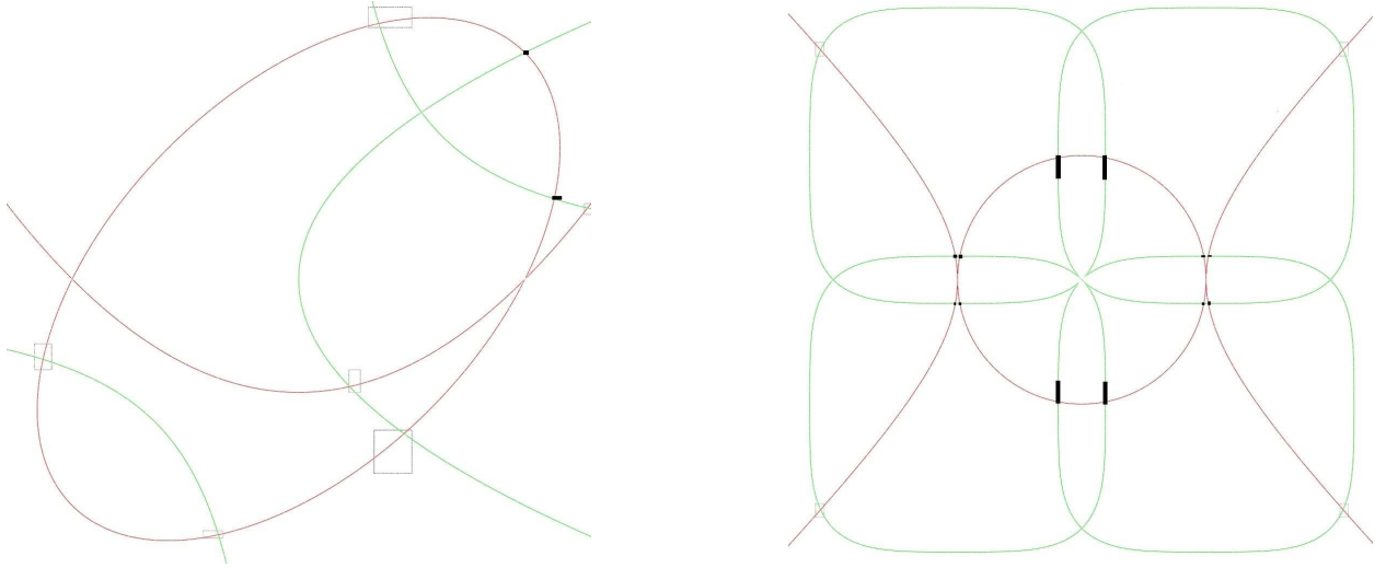
Figure 4: Isolating boxes of the real roots of the system Left: (\Sigma_3) , Right: (\Sigma_4) .
