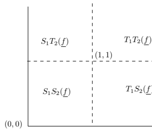
Figure 1: Subdividing the domain of \underline{f} .
