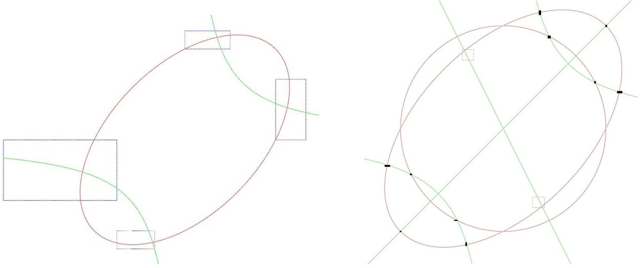
Figure 3: Isolating boxes of the real roots of Left: (\Sigma_1) , Right: (\Sigma_2) .
